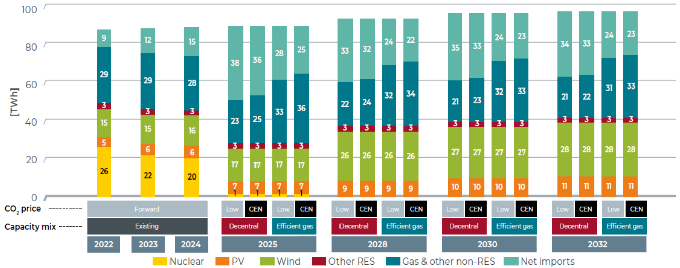
Figuur 11 Impact of capacity mix and CO2 prices on the future electricity generation mix in Belgium Elia, fig. 5-66, p.232
