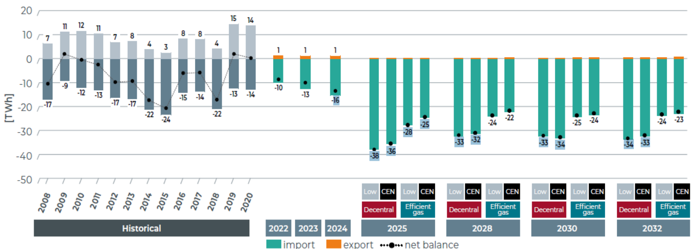
Figuur 12 Yearly imports/exports of electricity for Belgium in the 'central' scenario (for the 'decentral' and 'efficient gas' capacity mix combined with 'low' and 'central' CO2 prices), Elia, fig. 5-67, p.233
