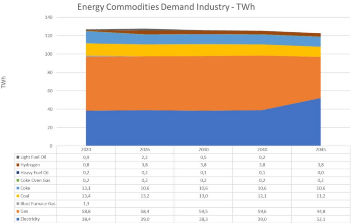
Figuur 16 Electricity demand Belgium, High Renewable Ambtion, Energyville(2020), Full presentation
