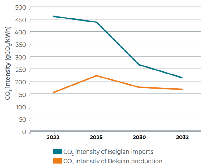
Figuur 20 CO 2 intensity of Belgian Production Park and imports, Elia (2021), fig. 5-72
